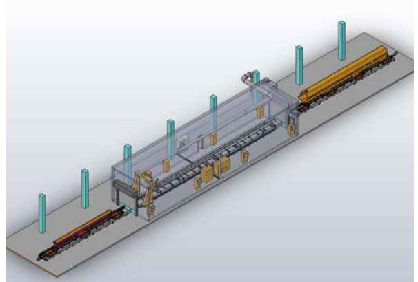
Layout of the 60 m long CLOOS laser hybrid system with the laser-proof cabin in the centre and the two loading and unloading stations which permit optimised work-piece flow.
